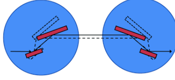
Figure 3: Optical layout of a four-crystal monochromator [?].
