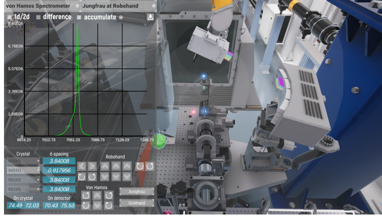
Figure 8: The Von Hamos spectrometer in operating position. with the read-out of the Jungfrau detector as well as the settings for the position to the left.
