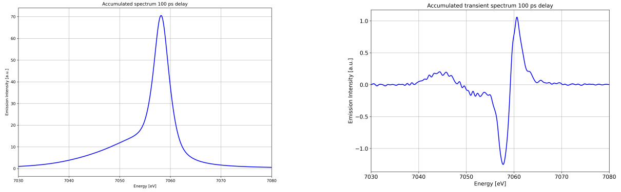
Figure 10: On the left the XES spectrum with the excitation laser on at a delay of 100 ps is plotted. On the right there's the difference spectrum at the same time delay.
