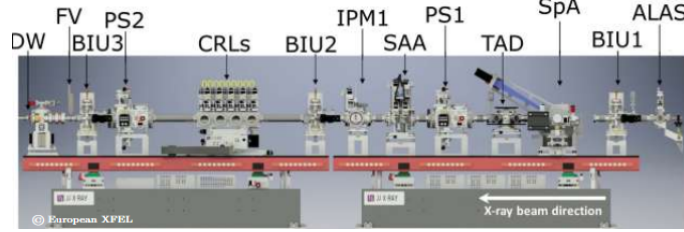
Figure 4: The optical bench in the FXE hut with the following components implemented: BIU 1,2,3 (beam imaging units), SpA (spectrum analyser), TAD (time arrival detector), PS 1,2 (power slits), SAA (solid attenuator assembly), IPM1 (intensity position monitor), CRLs (compound refractive lenses) [4].
